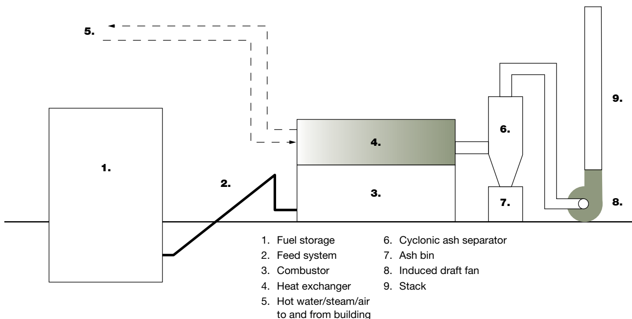
Major components of a commercial-scale biomass combustor system.
